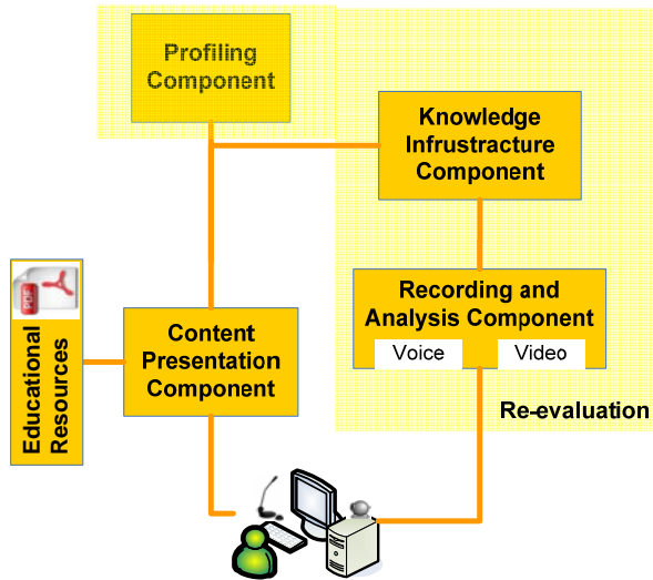
Figure 1: Intelligent Reading System's Architecture
