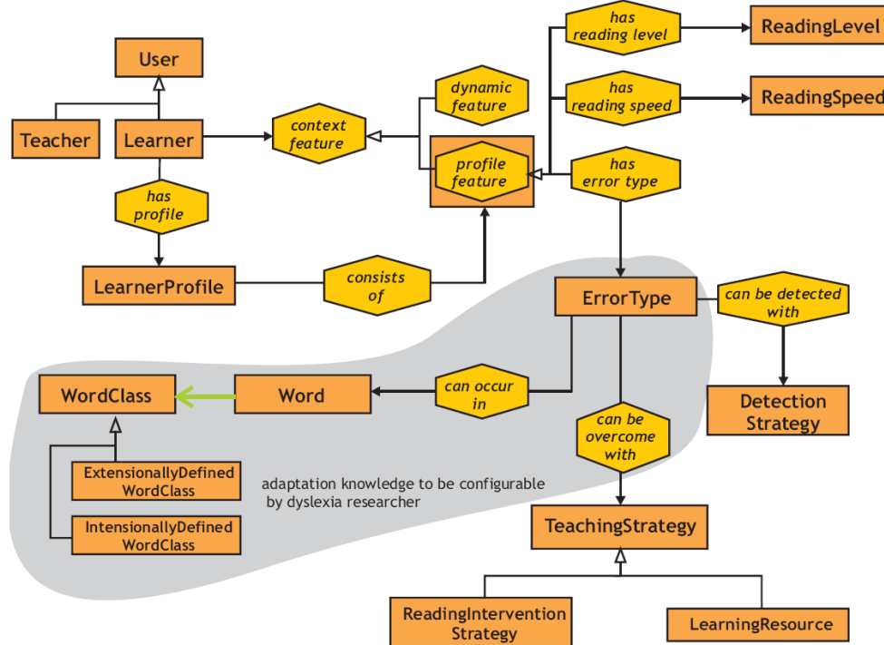
Figure 2: Part of the AGENT-DYSL Ontology
